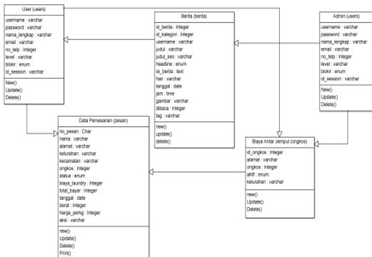
Gambar 5 Class Diagram
